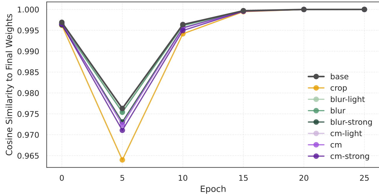
Convergence Speed of Backbones
